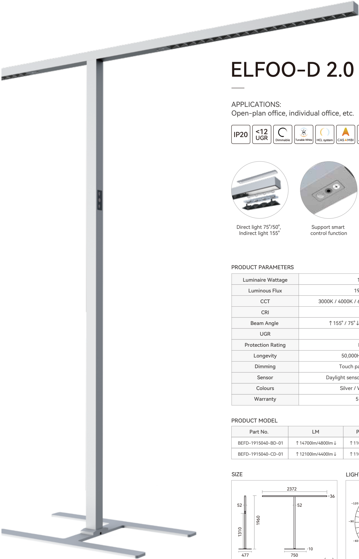
Direct and indirect light control individually
