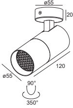
ALCH0131 Gu 10 Ceiling Surface Light
