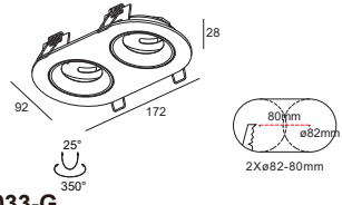
ALDL0033-G Gu10/Mr16 Downlight Cutout :2XØ82-80mm Optional :ALDL1401 ALDL1373
