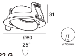
ALDL0122-G Gu10/Mr16 Downlight Cutout :Ø80mm Optional :ALDL1401 ALDL1373
