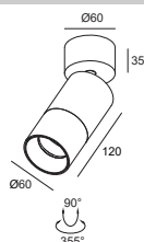
ALCH0201 Gu 10 Ceiling Surface Light
