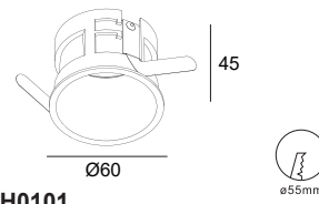
ALDH0101 Gu10/Mr16 Downlight Cutout :Ø55mm Optional :ALDL1401 ALDL1373
