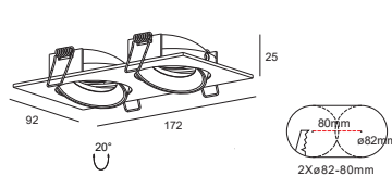
ALDL0031-G Gu10/Mr16 Downlight Cutout :2XØ82-80mm Optional :ALDL1401 ALDL1373
