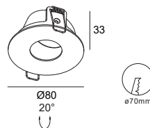
ALDH0104 Gu10/Mr16 Downlight Cutout :Ø70mm Optional :ALDL1401 ALDL1373
