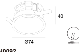
ALDH0092 Gu10/Mr16 Downlight Cutout :Ø68mm Optional :ALDL1401 ALDL1373 ALDL1022
