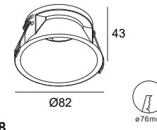
ALDH0048 Gu10/Mr16 Downlight Cutout :Ø76mm Optional :ALDL1401 ALDL1373 ALDL1022
