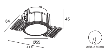
ALDH0102 Gu10/Mr16 Downlight Cutout :Ø75mm Optional :ALDL1401 ALDL1373 ALDL1022
