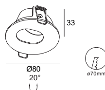
ALDH0105 Gu10/Mr16 Downlight Cutout :Ø70mm Optional :ALDL1401 ALDL1373
