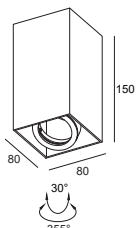
ALCH0179 Gu10/Mr16 Downlight CE IP20
