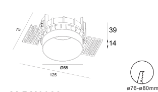
ALDH0088 Gu10/Mr16 Downlight Cutout :Ø76-ø80mm Optional :ALDL1401 ALDL1373 ALDL1022
